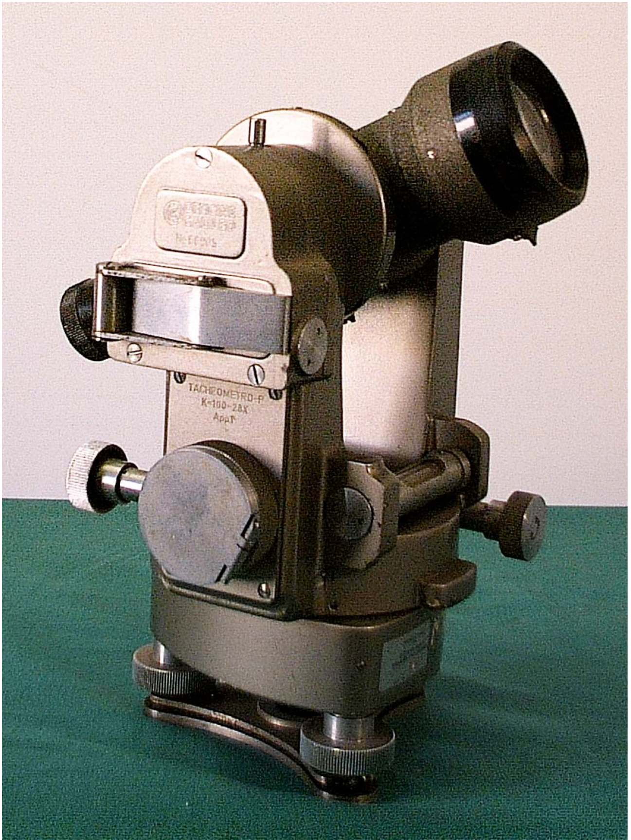
N° inventario 150 – Tacheometro Off. Galileo mod. P (1941)
