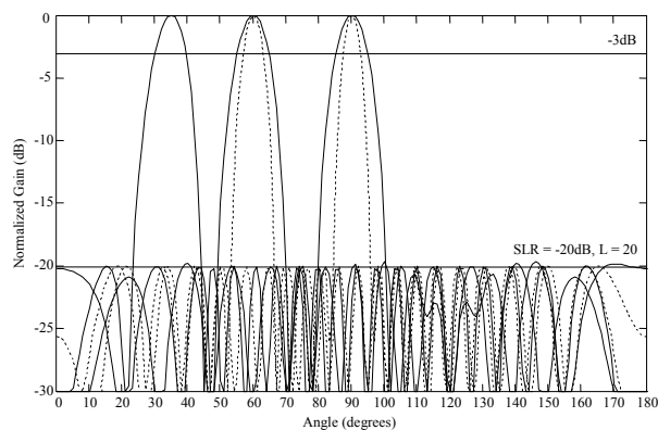
Figure 7 – Proposed and Chebyshev Patterns with ULA.
