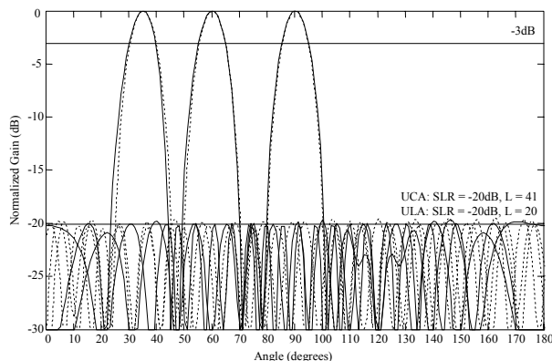
Figure 8 – Proposed Beampatterns with a ULA and Chebyshev Beampatterns with a UCA.
