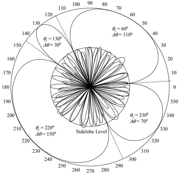
Figure 4 – Proposed Beampatterns (UCA, L = 35 ).
