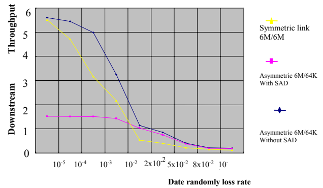
Chart 1: Uni-directional Single Flow Simulation on Loss Link
