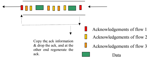
Figure 2: Illustration of SmartAckDropper(SAD)
