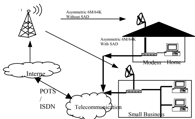
Figure 1: Network Topology with Asymmetric Links
