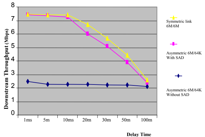
Chart 2: Uni-directional Single Flow Simulation on Delay Link
