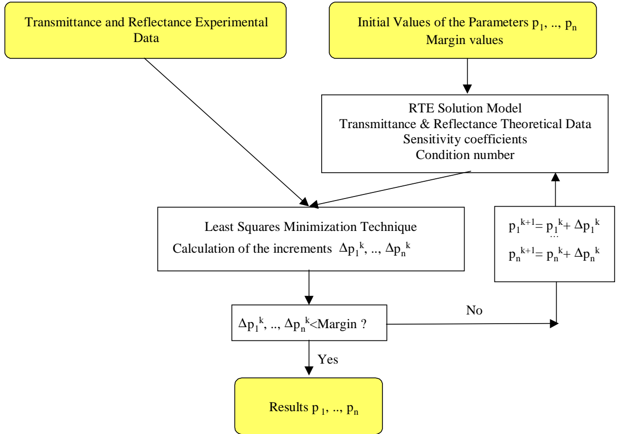
Fig. 1: Flow chart of the parameter identification procedure
