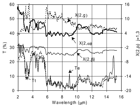
b) Bi-directional transmittance for direction 2 ( \mu=0.99948 ).
