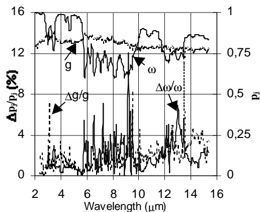
Fig. 7: Average and standard deviation of radiative properties calculated from 3 different thicknesses of sample [11]:
