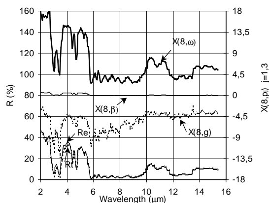
d) Hemispherical reflectance.
