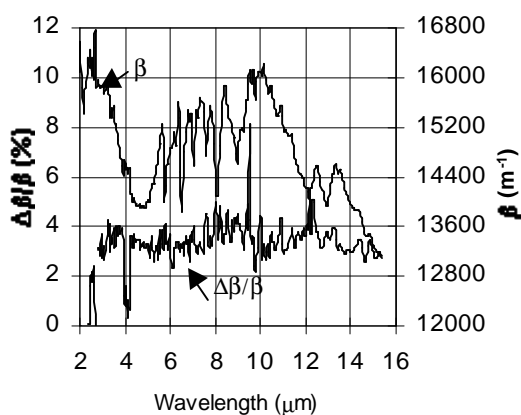
Fig. 7: Average and standard deviation of radiative properties calculated from 3 different thicknesses of sample [11]:
