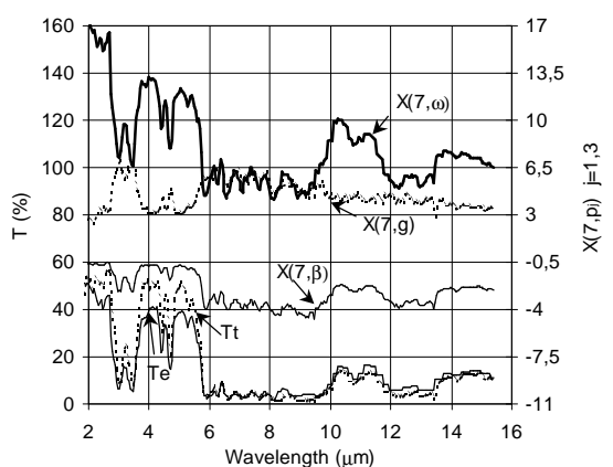
c) Hemispherical transmittance.
