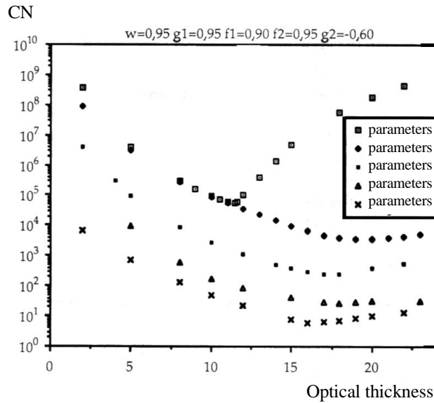
Fig. 5: Condition number as a function of optical thickness.
