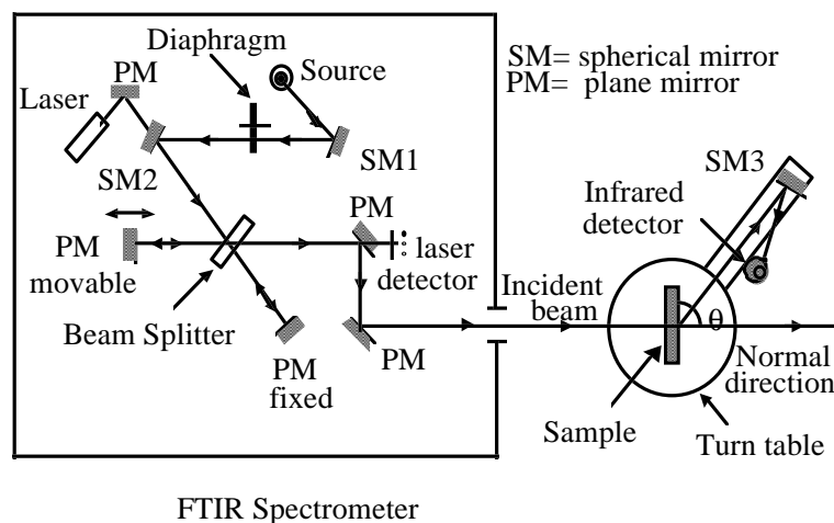
Fig. 2: BTDF/BRDF experimental set-up [16].
