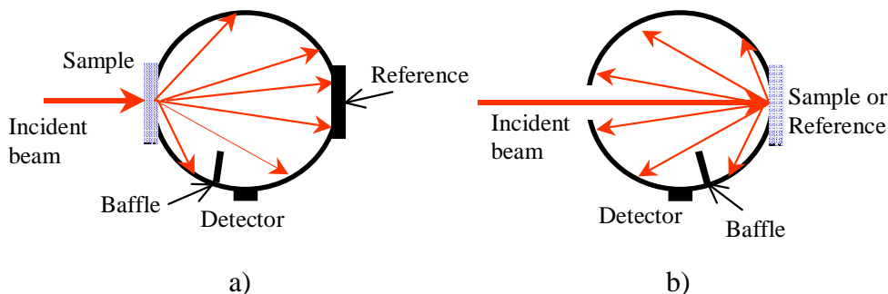
Fig. 3: Integrating sphere attachment of Bruker FTIR IFS 66v Spectrometer a) Directional-hemispherical transmittance b) Directional-hemispherical reflectance.
