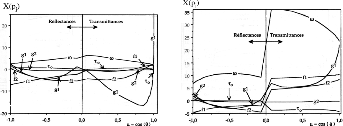
Fig 6: Normalized sensitivity coefficients. \omega=0.95, g_1=0.95, f_1=0.90, f_2=0.95, g_2=-0.6 . a) \tau_0=2 , b) \tau_0=20 .
