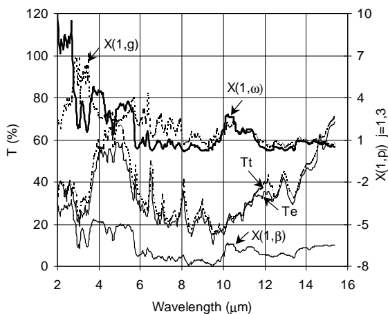
a) Bi-directional transmittance for direction 1 ( \mu=1 ).
