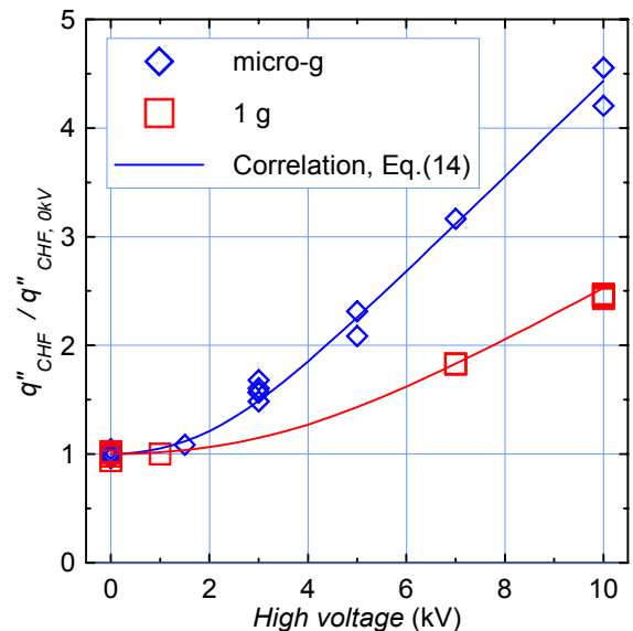
Fig. 11. Dimensionless (respect to the corresponding flux at 0 kV) critical heat flux at low g and on ground vs. the applied high voltage, for FC72.
