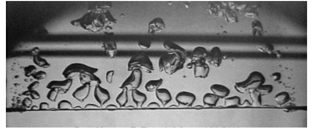
Fig. 15. Second film boiling regime, independent of applied voltage; monodimensional oscillatory pattern; p = 115 kPa; d = 0.2 mm; V = 7 kV; q = 850 kW/m 2 ; \Delta T_{sat} = 781 K.
