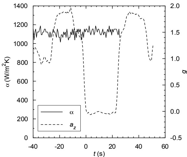
Fig. 3. Heat transfer coefficient and gravity acceleration for q = 21.3 \text{ kW/m}^2 , V = 3 \text{ kV} , FC72.
