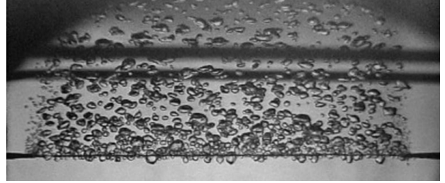
Fig. 14. EHD enhanced film boiling regime, multidimensional oscillatory pattern; p = 115 kPa; d = 0.2 mm; V = 7 kV; q = 400 kW/m 2 ; \Delta T_{sat} = 201 K.
