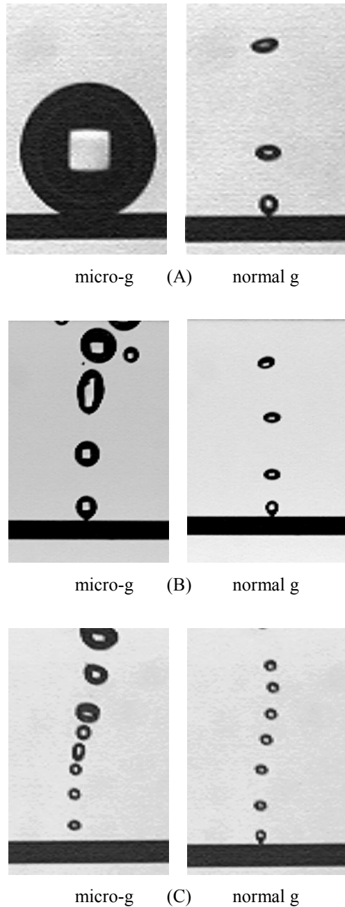
Fig. 17. Bubbling flow patterns in microgravity (left) and normal gravity (right) for: A) no electric field, B) 5 kV applied electric field, C) 15 kV applied electric field. The tube diameter (black line at the bottom) is 1 mm. Nitrogen bubbles in FC72, atmospheric pressure and ambient temperature (20 °C).
