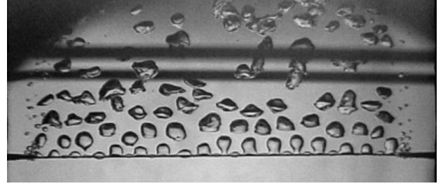
Fig. 13. First film boiling regime, monodimensional oscillatory pattern; p = 115 kPa; d = 0.2 mm; V = 0 kV; q = 400 kW/m 2 ; \Delta T_{sat} = 449 K.
