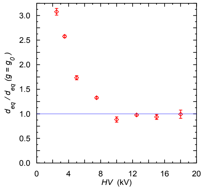
Fig. 18. Effect of applied electric field in micro gravity ( 10^{-4} g_0 ) on bubble detachment diameter (normalized to the value for the same field at normal gravity, g_0 ). Nitrogen bubbles in FC72, atmospheric pressure and ambient temperature (20 °C).
