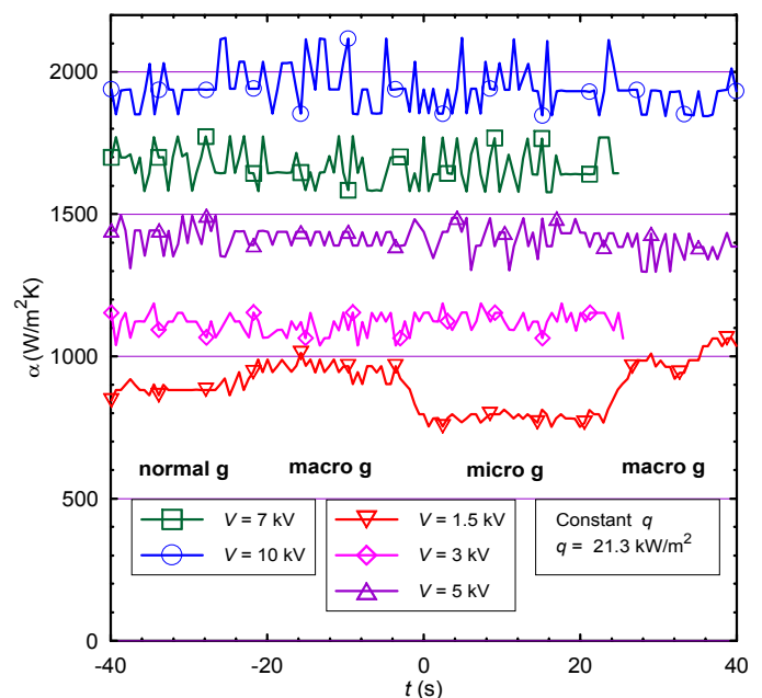
Fig. 4. Trend of the heat transfer coefficient vs. time (during a parabola) for different high voltage values. The low gravity phase is located within 0 and 20 seconds.
