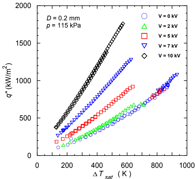
Fig. 12. Film boiling curves at different electric field levels.
