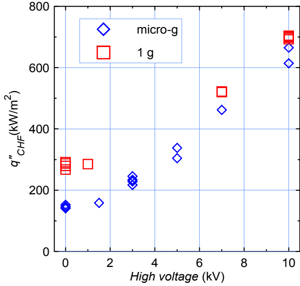
Fig. 10. Critical heat flux values vs. high voltage for FC72 on ground and in low gravity.
