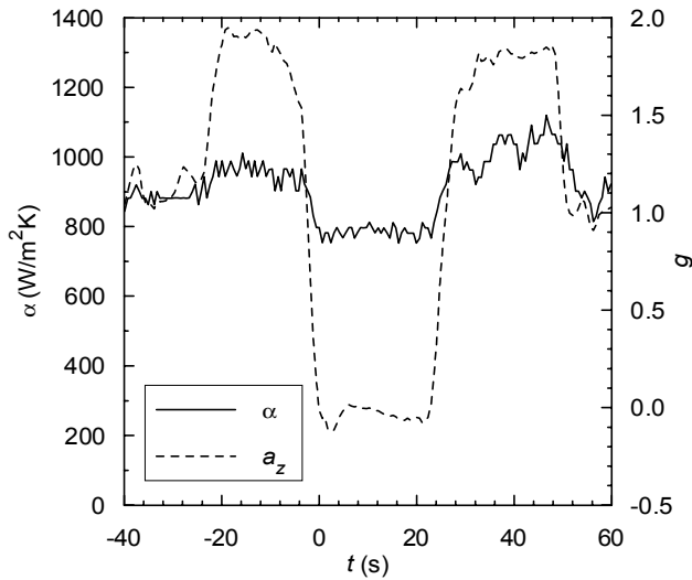
Fig. 2. Heat transfer coefficient and gravity acceleration for q = 21.3 \text{ kW/m}^2 , V = 1.5 \text{ kV} , FC72.
