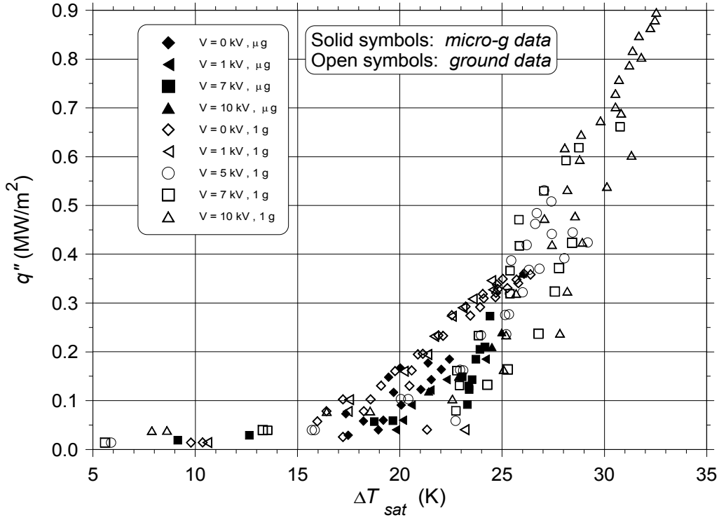
Fig. 7. Boiling curves in normal gravity and in low gravity for different applied voltages, R113, atmospheric pressure
