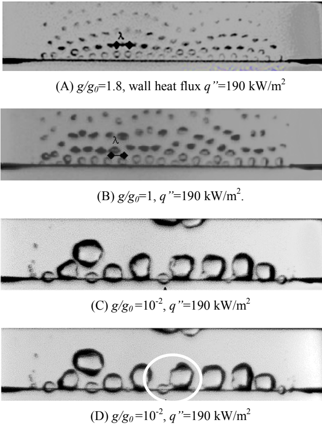
Fig. 16. Influence of gravity on vapor pattern in film boiling in slightly subcooled (3 K) FC72 at atmospheric pressure and zero electric field. Wire diameter 0.2 mm, length 47 mm. Gravity level and heat flux are indicated below each picture. Lateral coalescence phenomena are visible from (C) and (D) (e.g. white circle).
