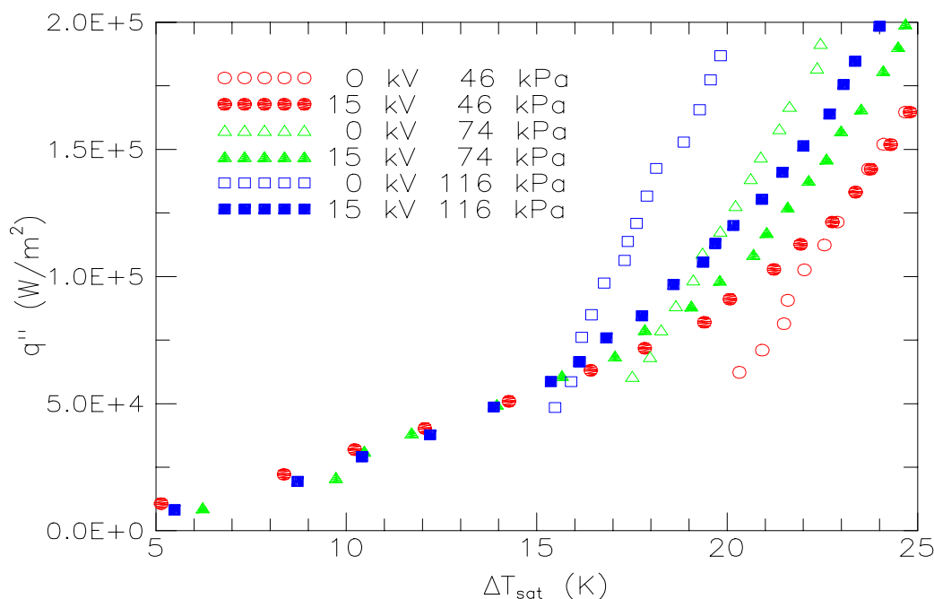
Fig. 6. Heat transfer coefficient at normal gravity for different pressure and applied electric fields. R113.
