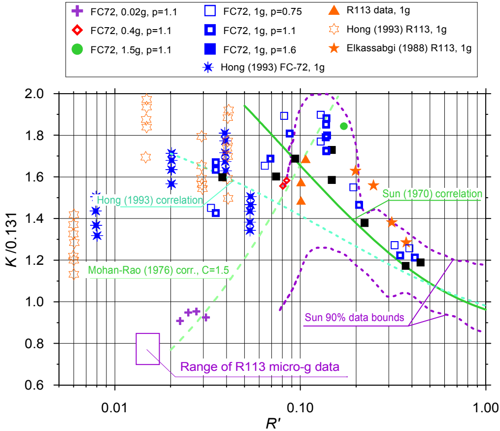
Fig. 9. Values of K in Eq. (8) and comparison with available correlations. All the data not countersigned with a reference belong to the present authors. The symbol p represents the system pressure in bar
