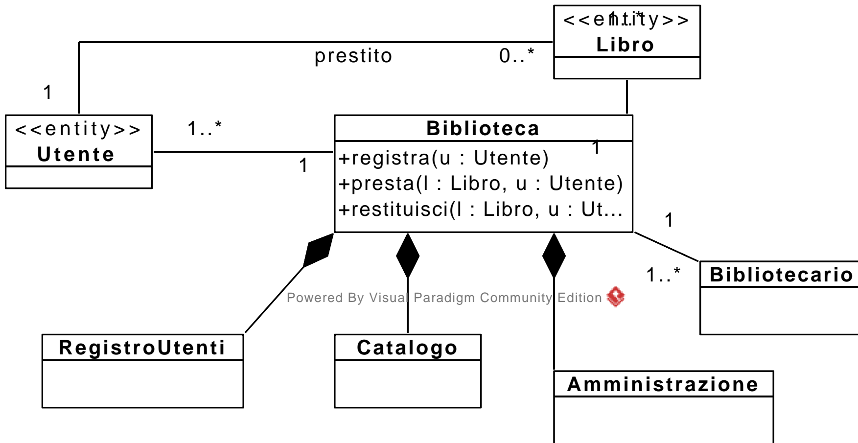
Class Diagram 1
