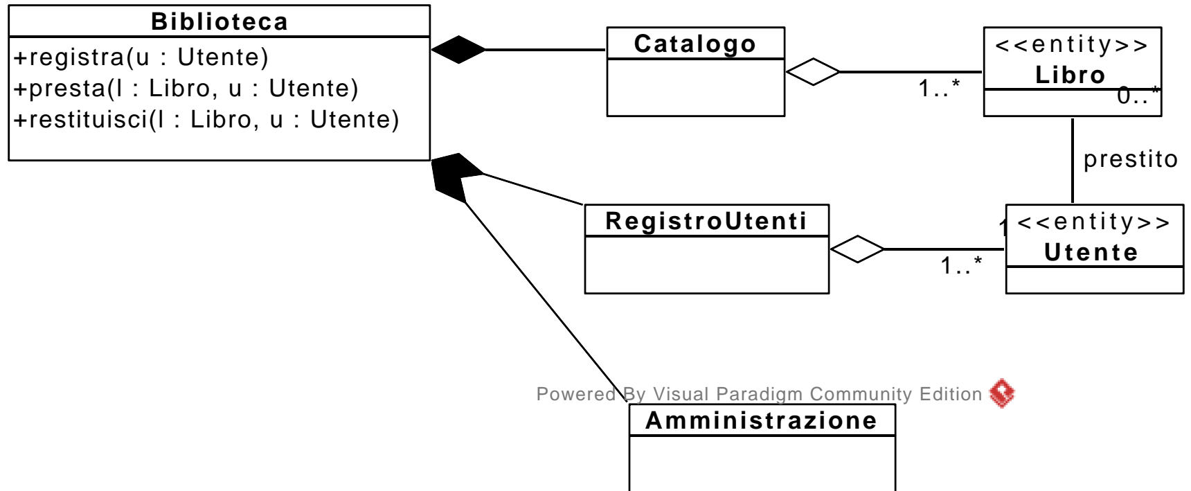
Class Diagram 2
